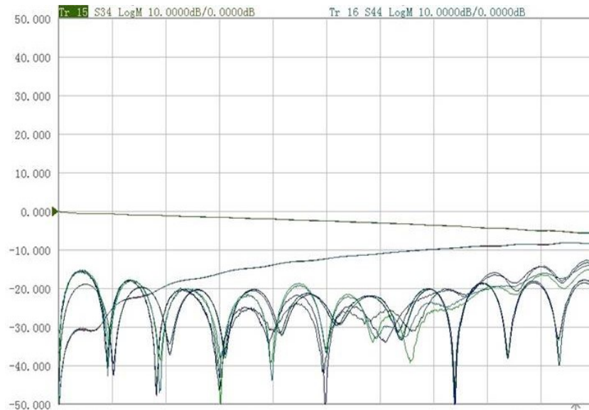
Before the fixture is embedded
